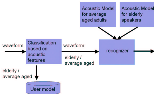
Figure 2: Serial account for speaker clustering
