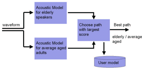
Figure 1: Parallel account for speaker clustering
